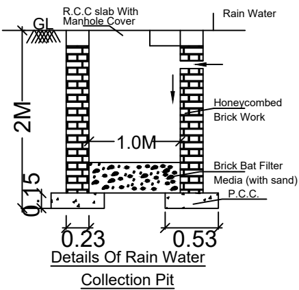
Details Of Rain Water Collection Pit
