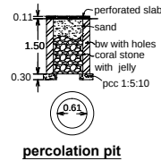
percolation pit
