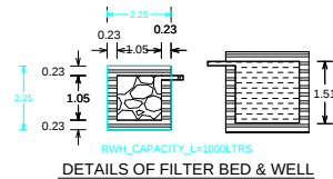
DETAILS OF FILTER BED & WELL
