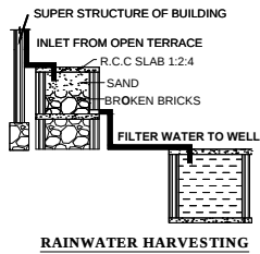
RAINWATER HARVESTING
