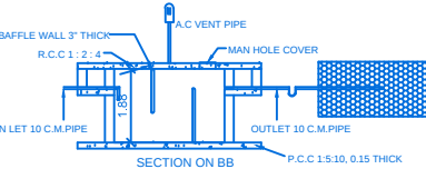
SECTION ON BB
