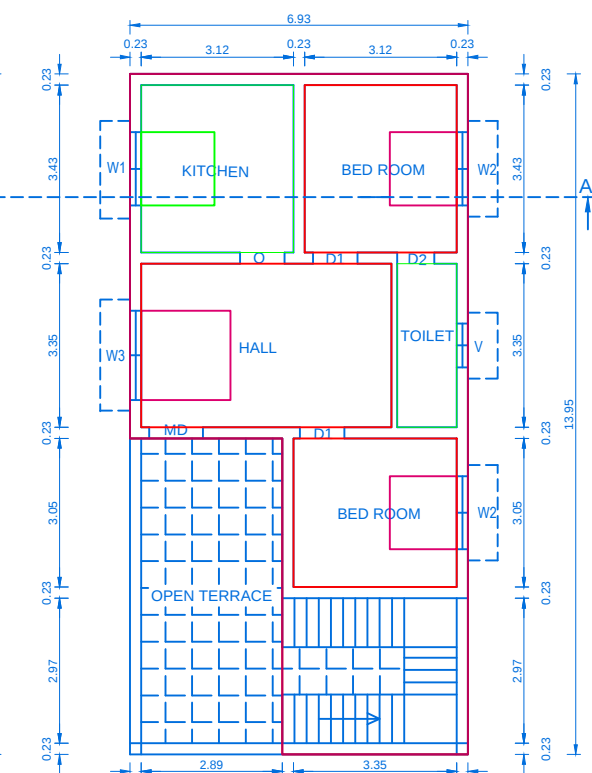
PROP.FIRST FLOOR PLAN
