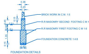
FOUNDATION DETAILS
