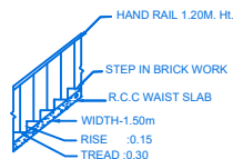
STAIR DETAIL
