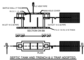
SEPTIC TANK AND TRENCH & U TRAP ADOPTED
