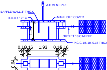
SEPTIC TANK & TRENCH
