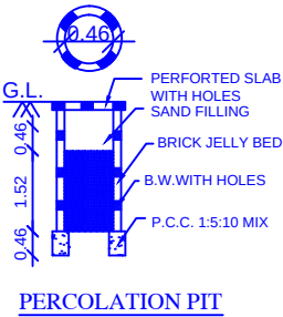
PERCOLATION PIT
