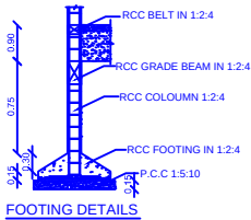
FOOTING DETAILS
