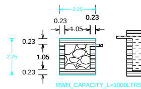
DETAILS OF FILTER BED & WELL
