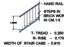
DETAILS OF STAIRCASE
