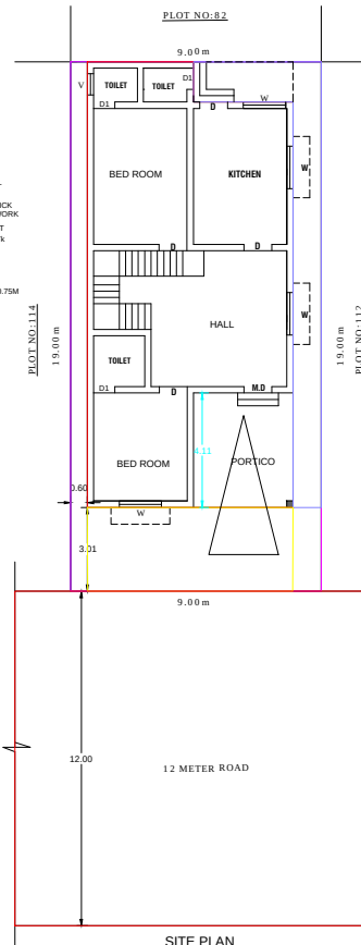
SITE PLAN SCALE (1:100)
