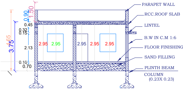
CROSS SECTION VIEW AB
