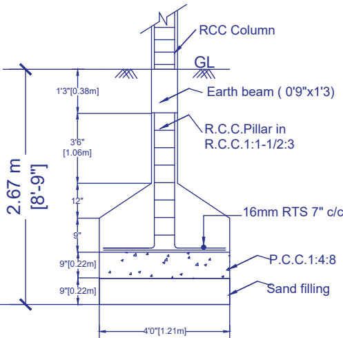
FOUNDATION DETAILS
