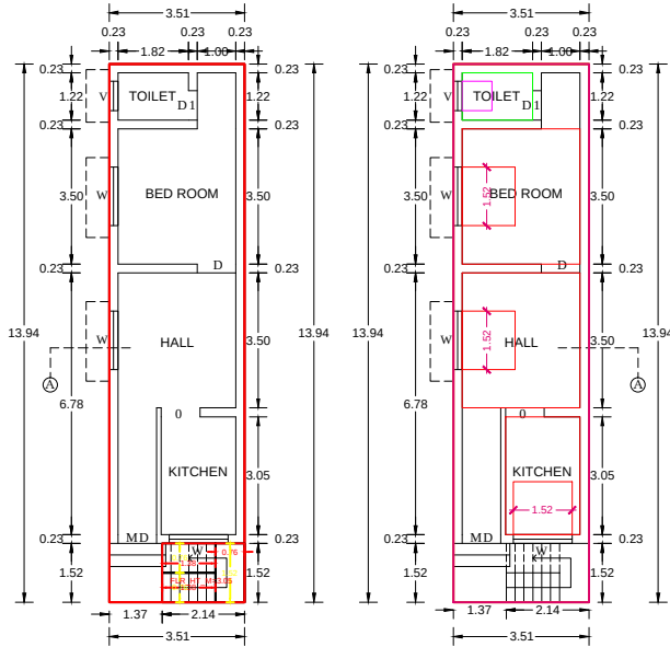
EXG.GROUND FLOOR PLAN
