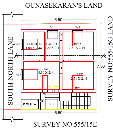
SITE PLAN CUM GROUND FLOOR PLAN
