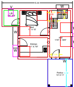
GROUND FLOOR
