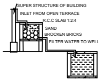
RAINWATER HARVESTING
