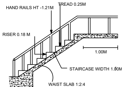
STAIRCASE DETAILS
