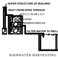
RAINWATER HARVESTING
