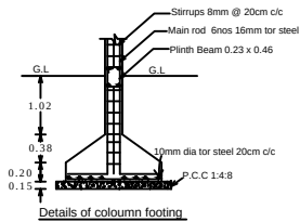
Details of column footing
