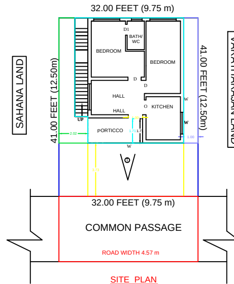
SITE PLAN
