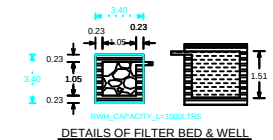
DETAILS OF FILTER BED & WELL
