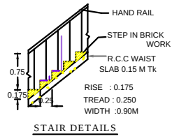
STAIR DETAILS
