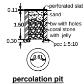
percolation pit
