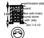
percolation pit
