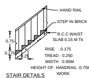
STAIR DETAILS
