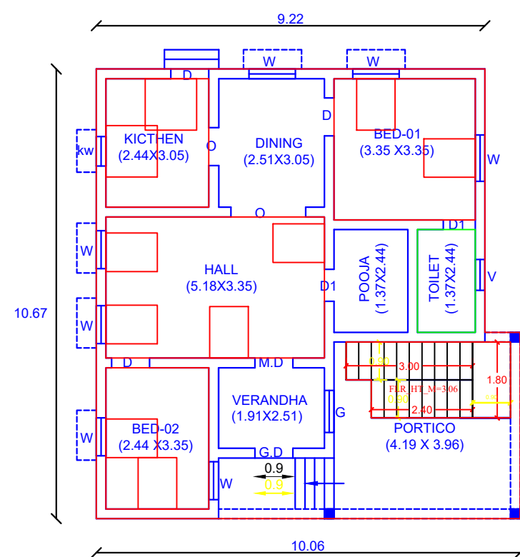
EXG.GROUND FLOOR PLAN
