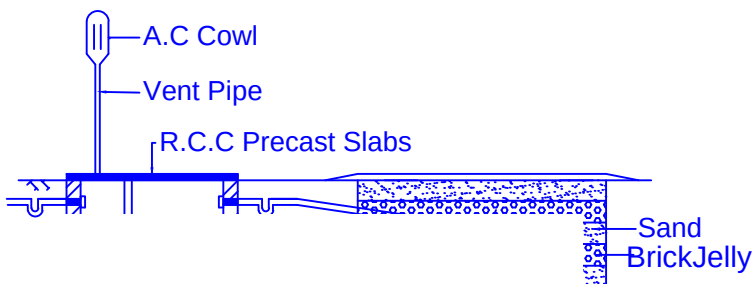
PLAN & SECTIONAL ELEVATION OF RAIN WATER HARVESTING
