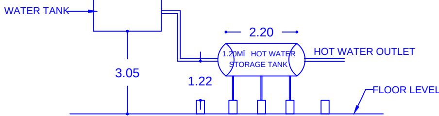
SOLAR WATER HEATING SYSTEM SWHS DETAILS
