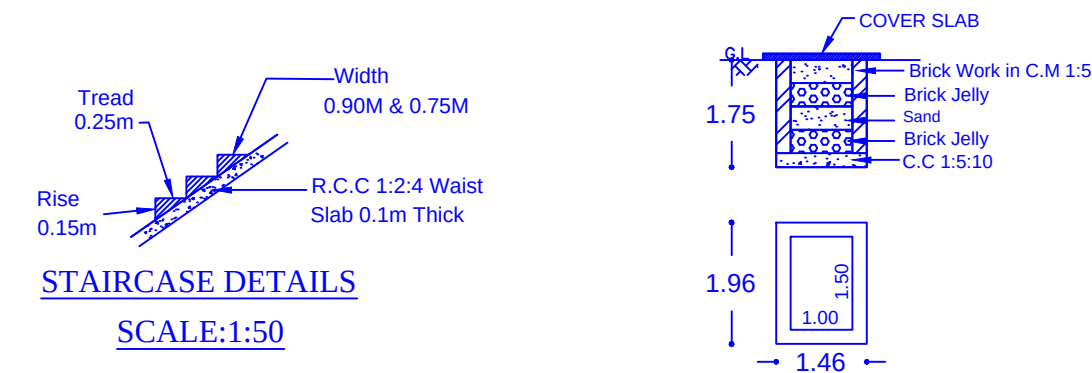
PLAN & SECTIONAL ELEVATION OF RAIN WATER HARVESTING
