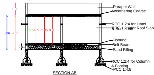
SECTION AB
