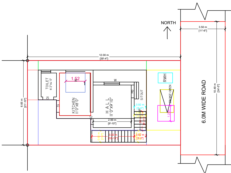
EXG., GROUND FLOOR PLAN
