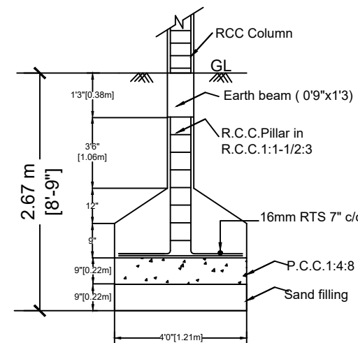
FOUNDATION DETAILS
