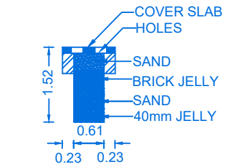
SECTION OF RAIN WATER COLLECTION TANK
