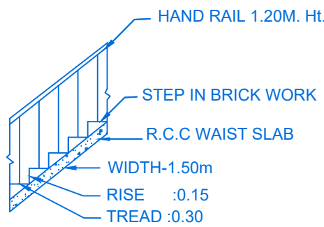
STAIR DETAIL
