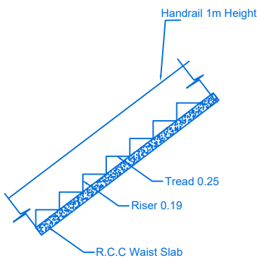
STAIR DETAILS
