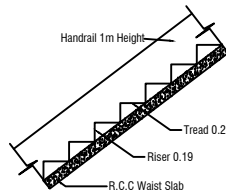
STAIR DETAILS
