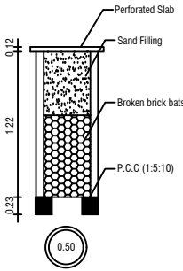
RAIN WATER COLLECTION WELL
