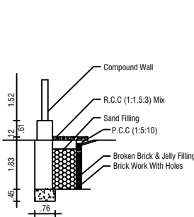
RAIN WATER HARVEST DETAILS
