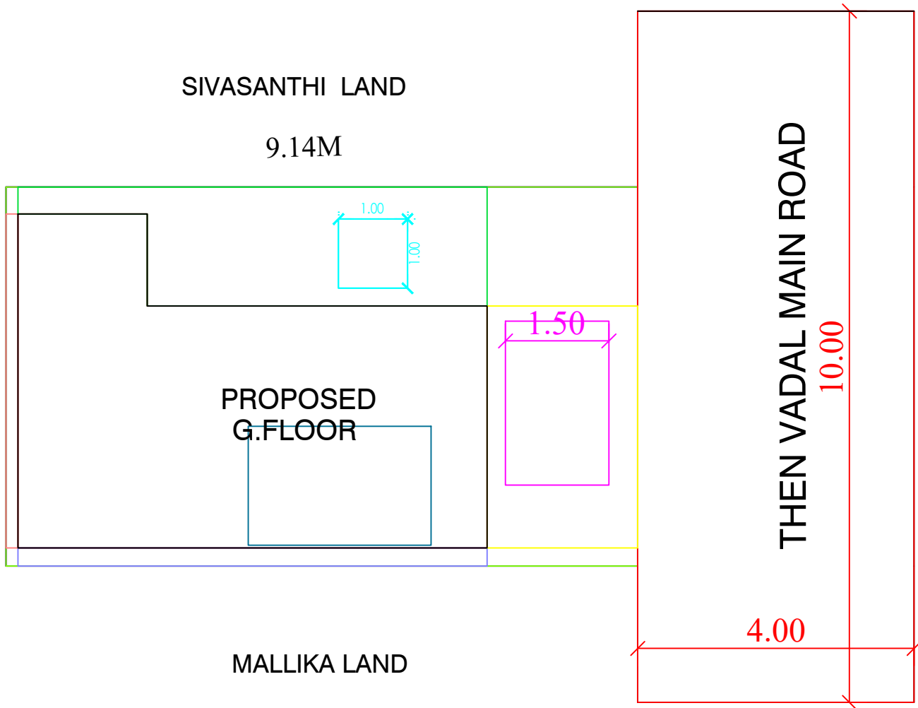
SITE PLAN
