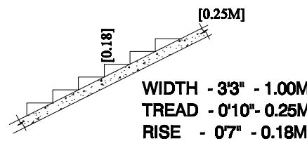
STAIRCASE DETAILS
