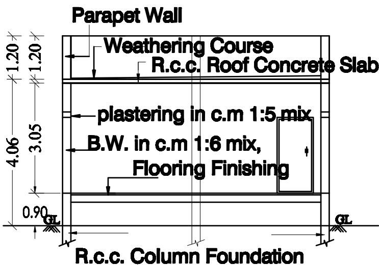
SECTION NN (SCALE: 1CM : 1M)
