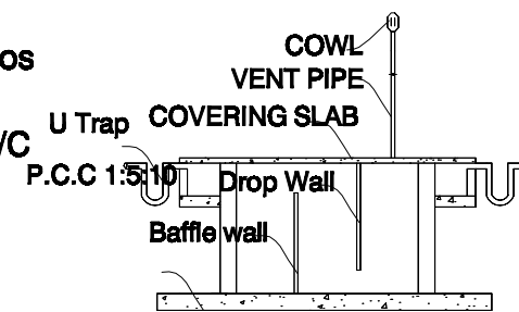
SECTION ON AB1
