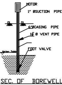
SEC. OF BOREWELL
