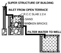
RAINWATER HARVESTING
