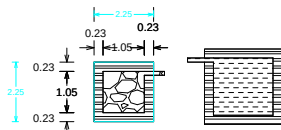
DETAILS OF FILTER BED & WELL
