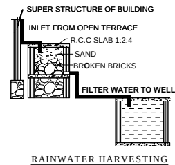
RAINWATER HARVESTING
