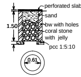
percolation pit
