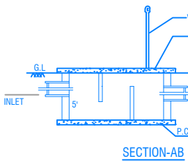
SECTION-AB
