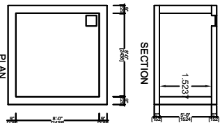
DETAILS OF COLLECTION SUMP FOR RAIN WATER HARVESTING OF ROOF TOP RAIN WATER RW/H_CAPACITY_L=5000LTRS
