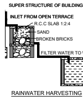
RAINWATER HARVESTING
