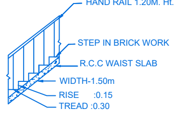
STAIR DETAIL
