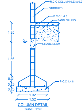
COLUMN DETAIL (SCALE 1:50)
