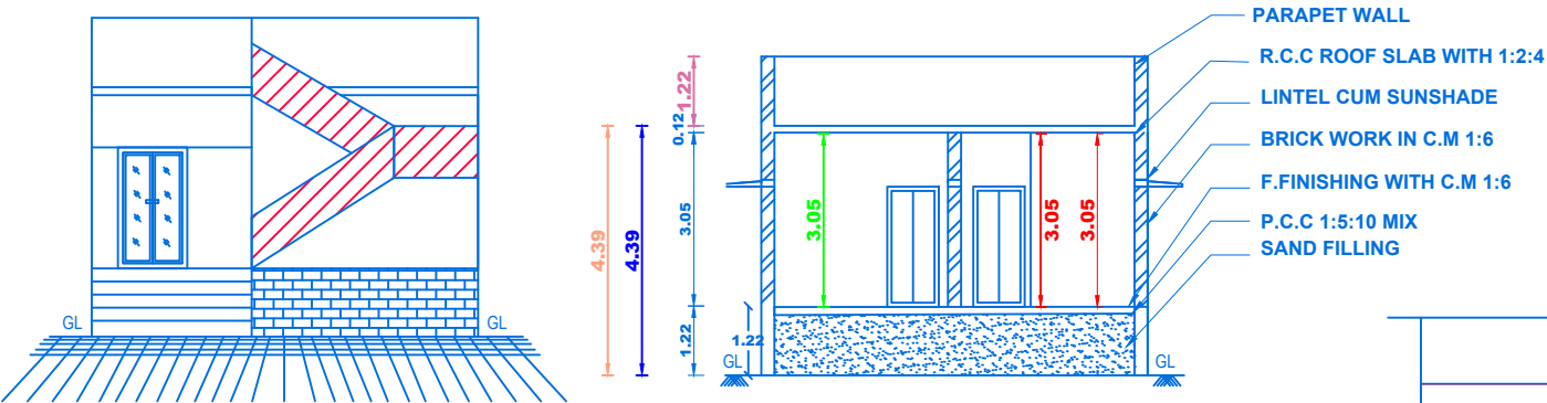
FRONT ELEVATION
