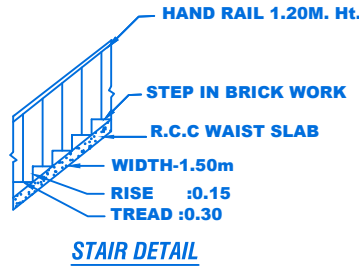
STAIR DETAIL
