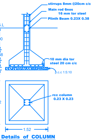
Details of COLUMN
