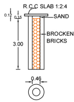
PERCOLATION PIT
