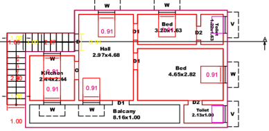
PROPOSED FIRST FLOOR PLAN
