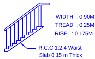
STAIRCASE SECTION
