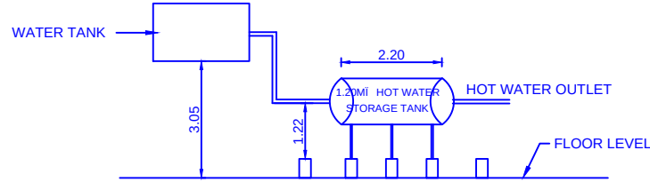
SOLAR WATER HEATING SYSTEM SWHS DETAILS
