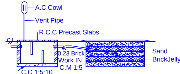
SECTION ON "BB" 'U' TROP MODEL S.T.ADOPTED
