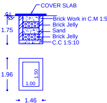
PLAN & SECTIONAL ELEVATION OF RAIN WATER HARVESTING
