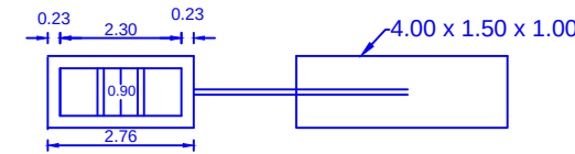
PLAN OF SEPTIC TANK & DISPERSION TRENCH
