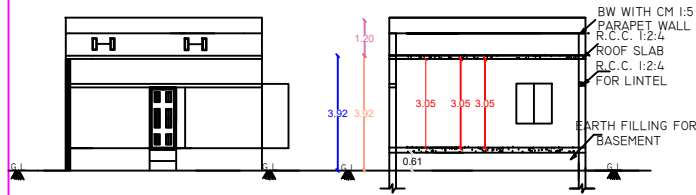
FRONT ELEVATION
