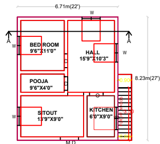
PROPOSED GROUND FLOOR
