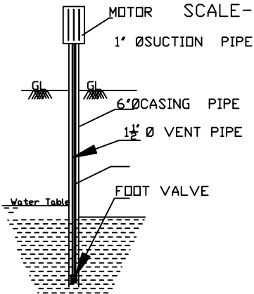
SEC. OF BOREWELL
