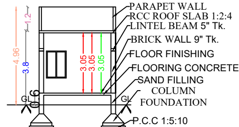
SECTION ON B-B
