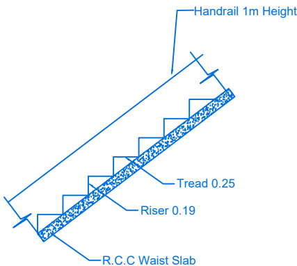
STAIR DETAILS
