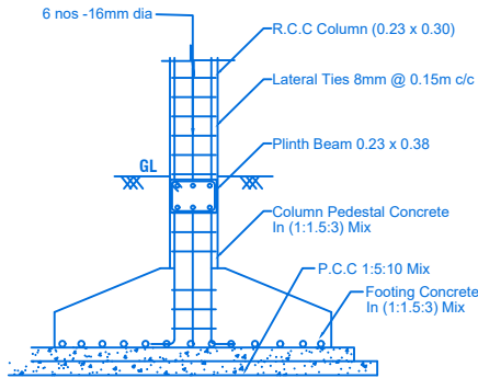
COLUMN FOOTING DETAILS
