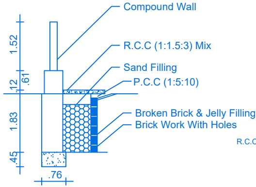
RAIN WATER HARVEST DETAILS
