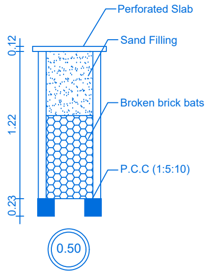
RAIN WATER COLLECTION WELL
