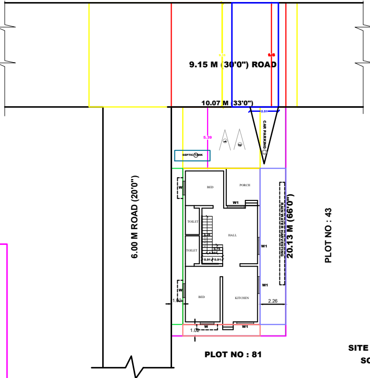
TOPO SKETCH
