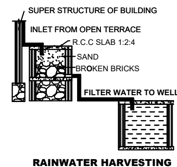
RAINWATER HARVESTING
