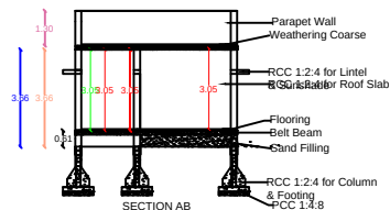
SECTION AB
