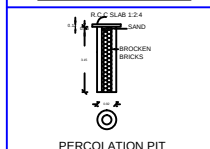
PERCOLATION PIT
