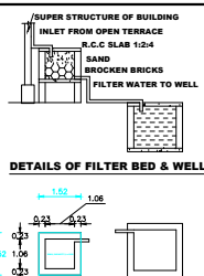
RAIN WATER HARVESTING
