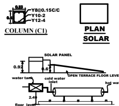
Details of solar water heating system
