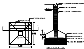
SECTION AT XX
