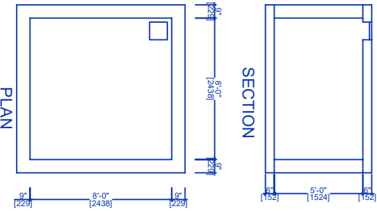
DETAILS OF COLLECTION SUMP FOR RAIN
