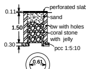
percolation pit
