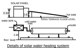
Details of solar water heating system
