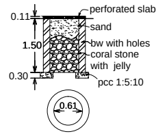
percolation pit
