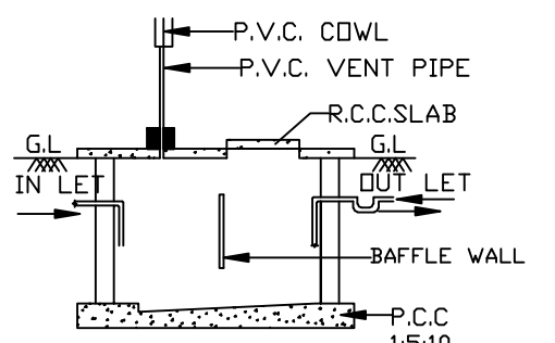
SEC. OF SEPTIC TANK
