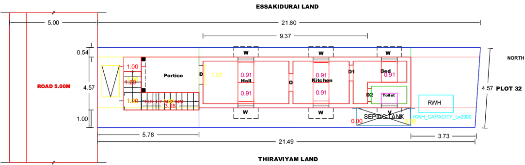
SITE PLAN FOR THE PROPOSAL
