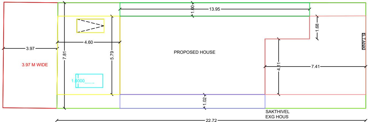
SITE PLAN
