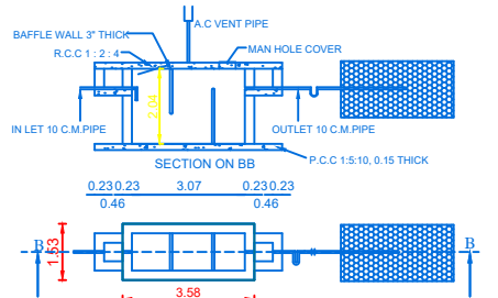
SEPTIC TANK AND TRENCH & U TRAP ADOPTED
