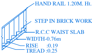
STAIR DETAIL
